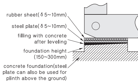
Foundation sketch
