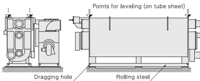
Leveling sketch
